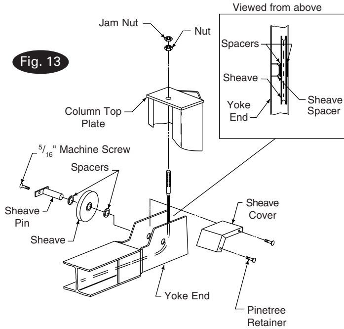
Attaching Cables
