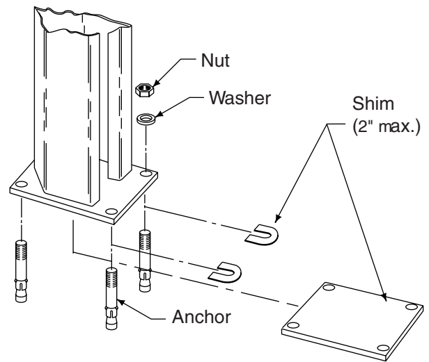
Shimming Column
