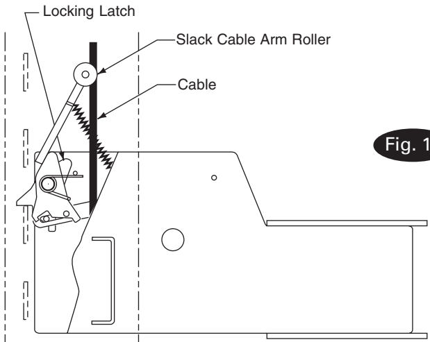
Cable in Slack Cable Arm Rollers
