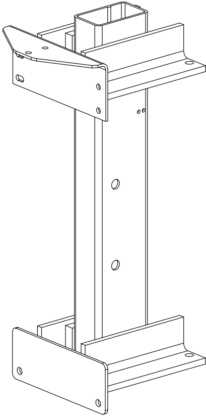
TP10-7100 Top Bracket Weld (2)
