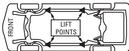
Perimeter Frame
